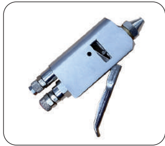
Bactericide dispensing gun (standard)
