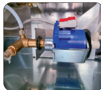
Electromagnetic pump (standard)
